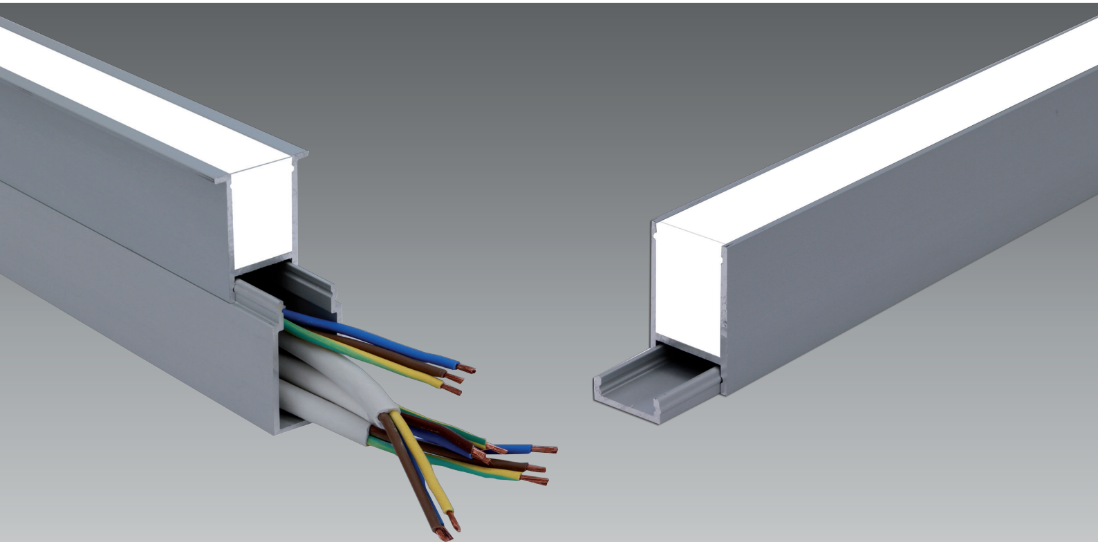
Example for EA-3 with cable channel AKF-3 example for EA-3 with cable conduit AKF-3
